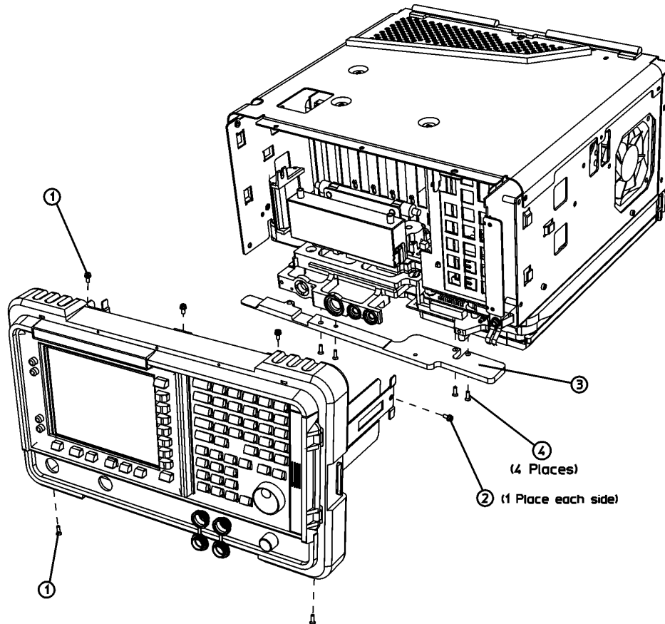
Figure 23 Front Frame Assembly Replacement
